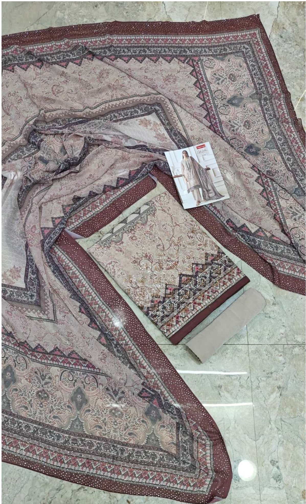
Star Galaxy #2530
