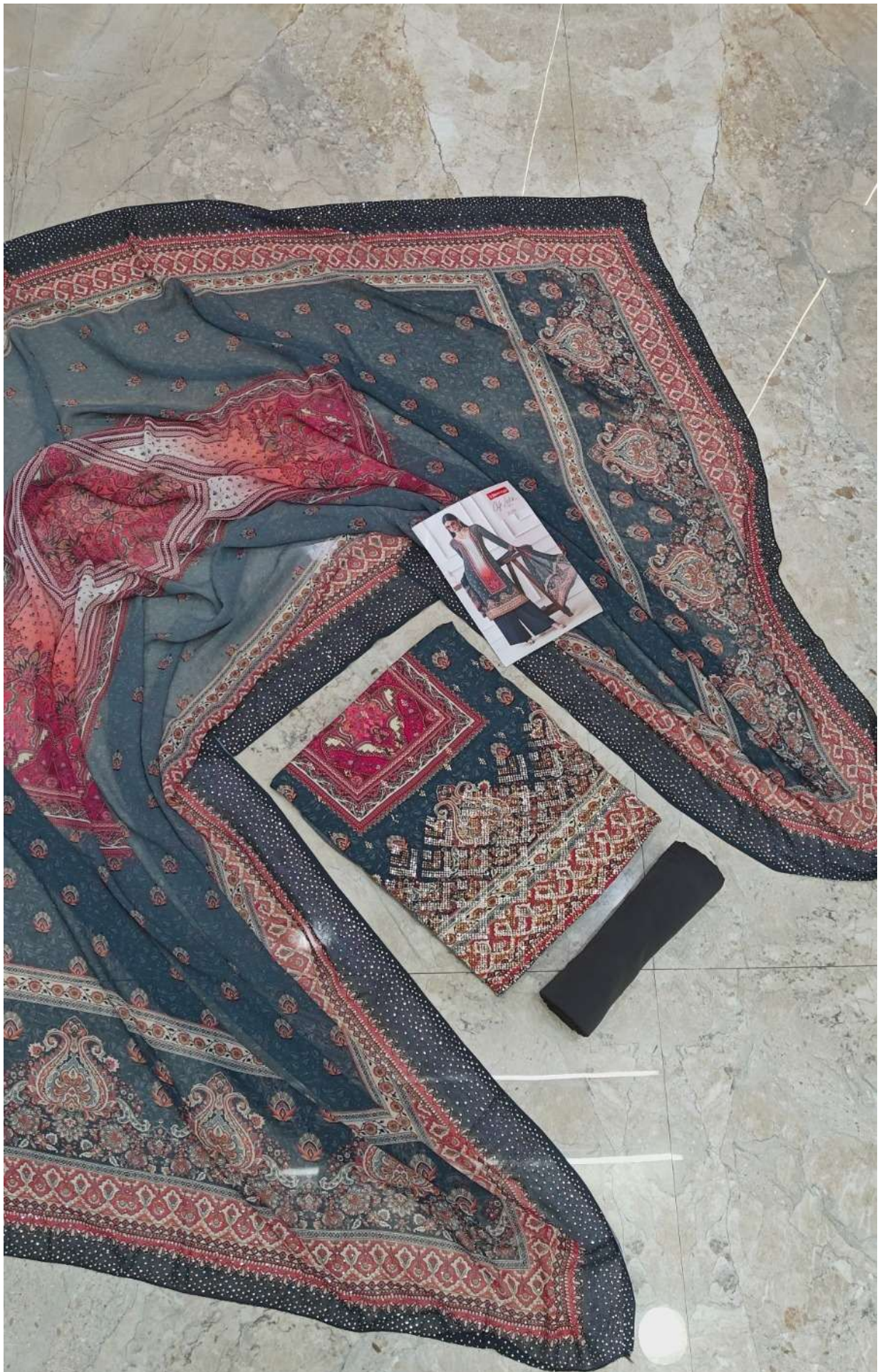
Star Galaxy #2532
