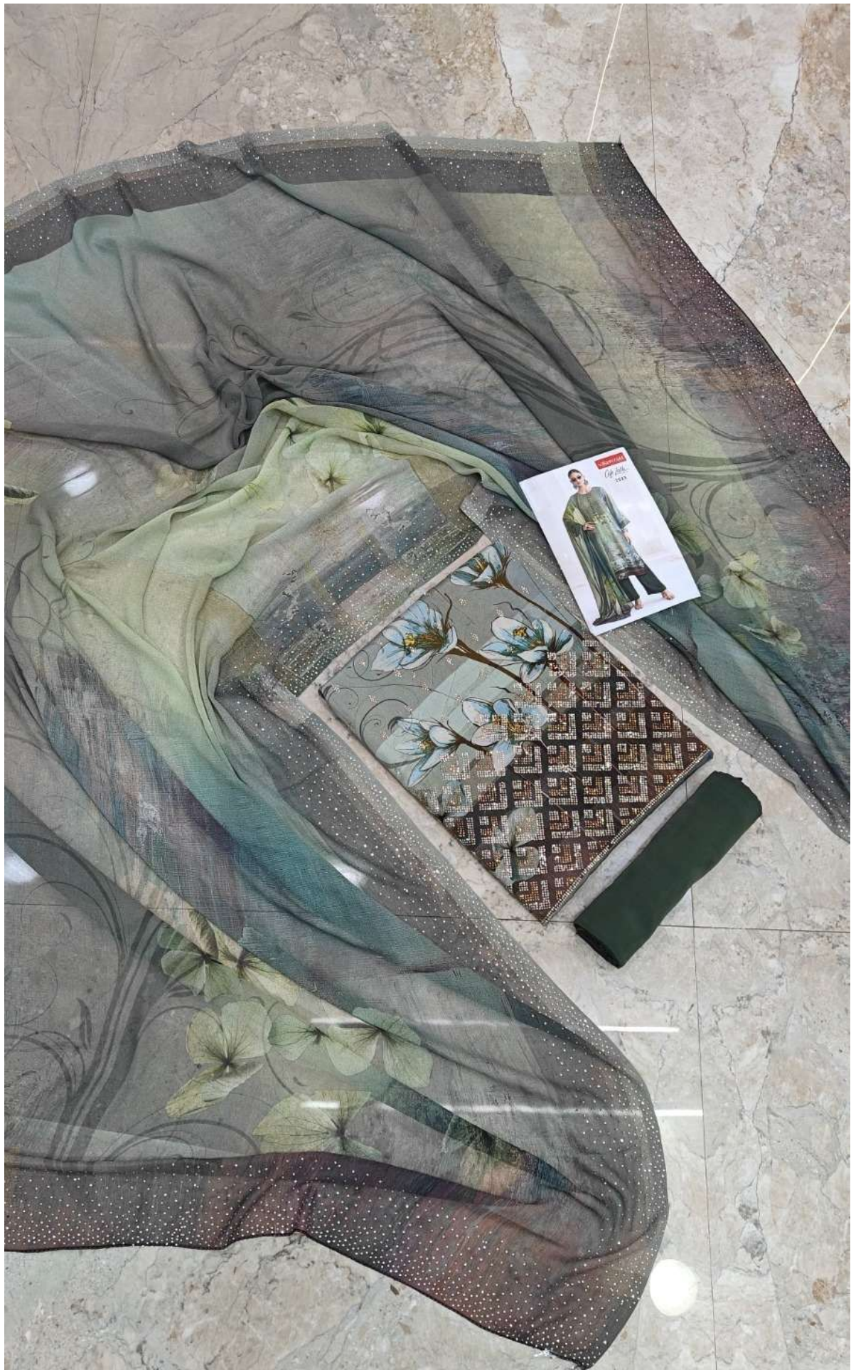
Star Galaxy #2523
